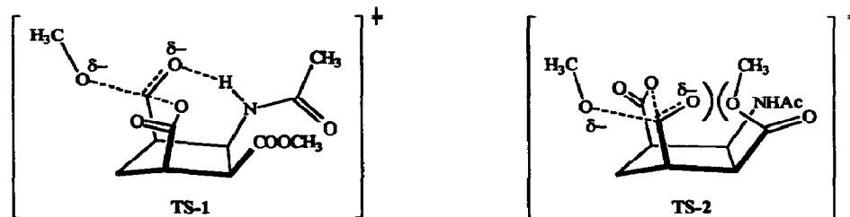
Figure 1: Transition structures for the reaction of methoxide anion with acetyl analogue of anhydride 6.
